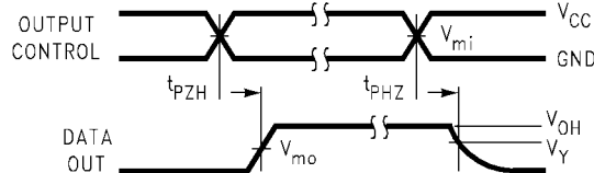
FIGURE 7. 3-STATE Output High Enable and Disable Times for Low Voltage Logic
